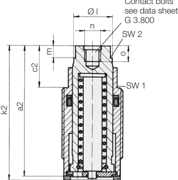
Version with female thread
