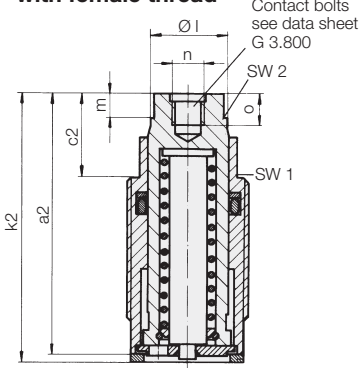
Version with female thread
