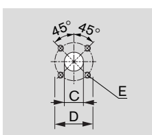
20 Rectangular flange
