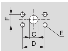
07 Square flange SAE, thread, metric
