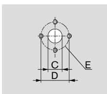
30 Rectangular flange
