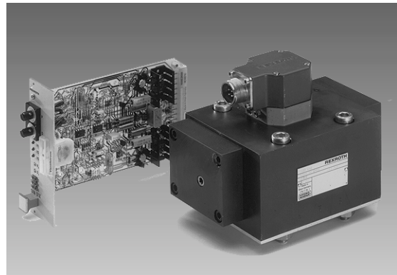
Type 4WS2EM 16-2X/...B... with mechanical feedback and associated external control electronics (separate order)
