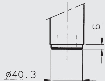
Weld model
