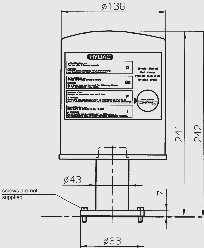
Flange model
