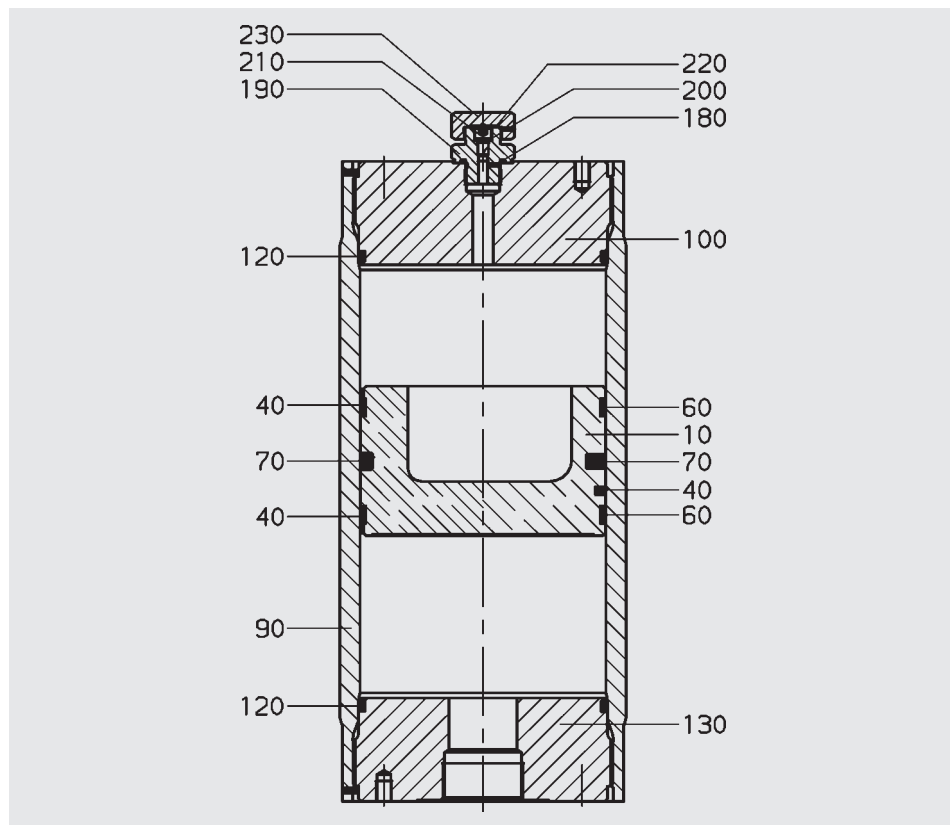
Complete piston (Table 8)
